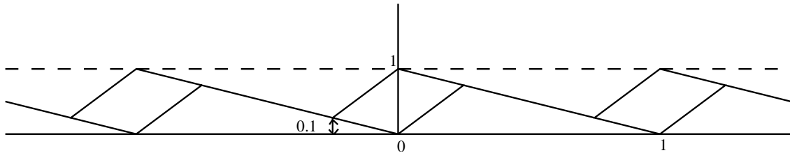
The kite-like function \alpha_0
