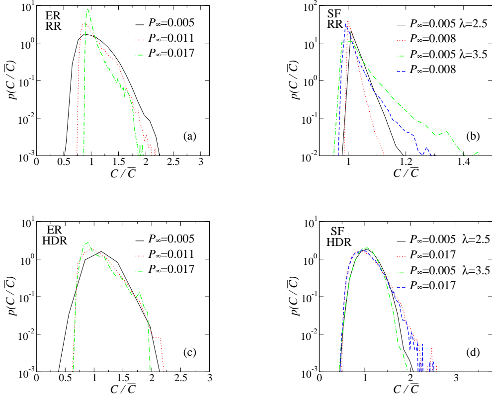
FIG. 3: Probability distributions p(C/\bar{C}) versus C/\bar{C} for several values of P_\infty and for ER networks with \langle k \rangle = 3 , N = 200000 and SF networks with N = 80000 and \lambda = 2.5 and 3.5 . (a) RR strategy on ER networks, (b) RR strategy on SF networks, (c) HDR strategy on ER networks and (d) HDR strategy on SF networks.
