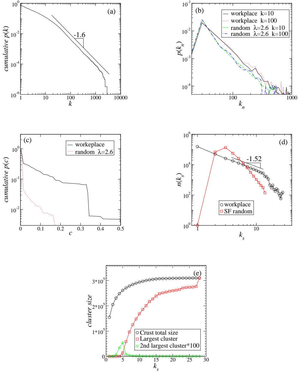
FIG. 5: Properties of the Swedish network of workplaces. (a) The cumulative degree distribution (showing \lambda = 2.6 ). (b) The distribution of k_n , the degree of the neighbors of nodes having degree k . (c) The cumulative distribution of clustering coefficient c . (d) Number of nodes in shell k_s . (e) Size of largest and second largest cluster in each k -crust. In (b), (c) and (d) the distributions of random SF networks with the same \lambda and N are plotted for comparison.
