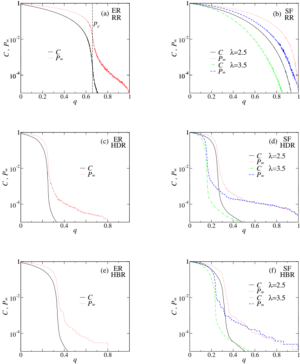
FIG. 1: The behavior of C and P_\infty versus q on ER and SF networks. For ER networks, N = 200000 and \langle k \rangle = 3 . For SF networks, N = 80000 . The graphs are (a) RR strategy on ER networks, (b) RR strategy on SF networks, (c) HDR strategy on ER networks, (d) HDR strategy on SF networks, (e) HBR strategy on ER networks and (f) HBR strategy on SF networks.
