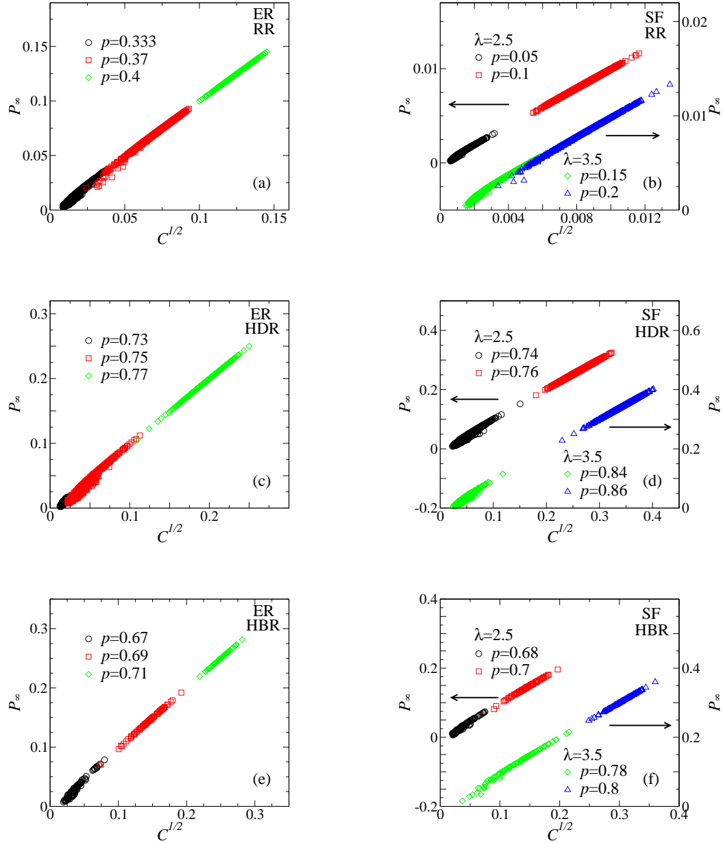
FIG. 2: Relationship between C^{1/2} and P_{\infty} for ER and SF networks with system size N = 50000 . For ER networks, the average degree \langle k \rangle = 3 , and for SF networks, \lambda = 2.5 and 3.5 . The graphs are (a) RR strategy on ER networks, (b) RR strategy on SF networks, (c) HDR strategy on ER networks, (d) HDR strategy on SF networks, (e) HBR strategy on ER networks and (f) HBR strategy on SF networks.
