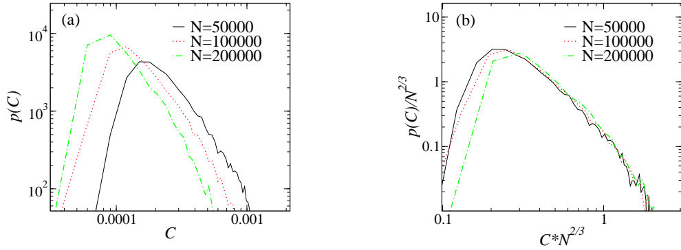
FIG. 4: The dependence of p(C) on the system size N with p = p_c for (a) before scaling and (b) after scaling. Simulations are performed on ER networks with \langle k \rangle = 3 .
