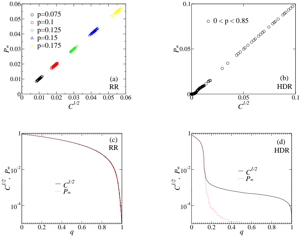
FIG. 6: P_\infty vs C^{1/2} for (a) RR strategy and (b) HDR strategy and plot C^{1/2} , P_\infty versus q for (c) RR strategy and (d) HDR strategy for the Swedish network of workplaces with N = 310136 nodes.
