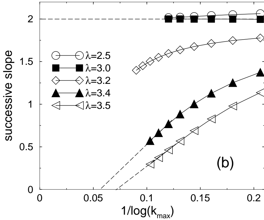
FIG. 5: (a) \log c_0 as a function of \log(k_{\max}) . (b) Plot of the successive slopes of (a) as a function of 1/\log(k_{\max}) .
