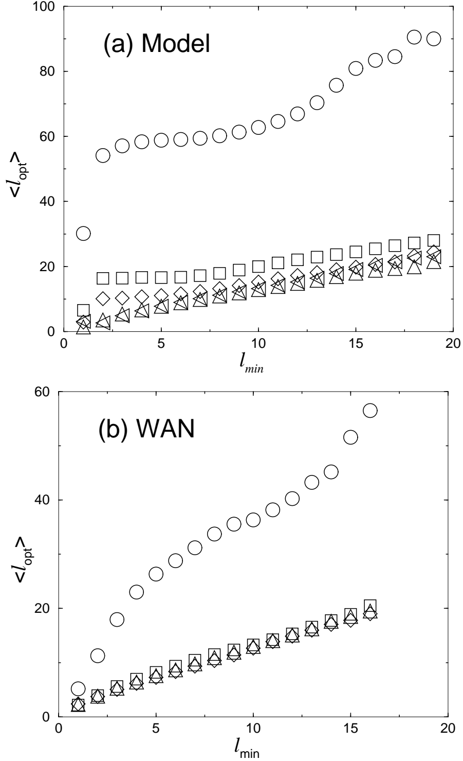
FIG. 7: (a) Plot of \langle l_{\text{opt}} \rangle as a function of l_{\text{min}} for our model of correlated weighted SF network with \lambda = 2.5 , in the SD limit ( \circ ), \alpha = 2 ( \square ), \alpha = 1 ( \diamond ), \alpha = 0 ( \triangle ) and \alpha = -1 ( \triangleleft ). (b) Same plot as in (a) for the real WAN network with \alpha = 1 ( \circ ), \alpha = 0 ( \square ), \alpha = -1 ( \diamond ) and \alpha = -0.5 ( \triangle ).
