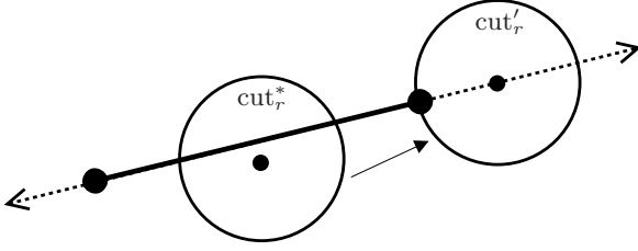
Fig. 15. An example illustrating the observation in Lemma 8. \text{cut}_r' is a translated version of \text{cut}_r^* such that [x', y'] lies on the line which contains the intersected link and \text{cut}_r' intersects the link at exactly one point (recall [x', y'] is the center of \text{cut}_r' ).
