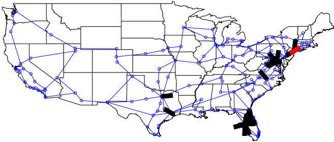
Fig. 19. Line segments cuts optimizing TEC for h = 2 - the red cuts maximize TEC and the black lines are nearly worst-case cuts.
