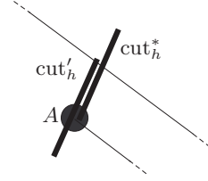
Fig. 12. Translate \text{cut}_h^* along the line which contains it until one of its endpoints intersects a link; we call this new cut \text{cut}'_h . \text{cut}'_h intersects all links \text{cut}_h^* intersects.
