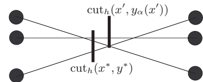
Fig. 9. \text{cut}_h(x^*, y^*) is a worst-case cut and has a unique (i_\omega, j_\omega) and (i_\alpha, j_\alpha) . From this we are able to find \text{cut}_h(x', y_\alpha(x')) , a worst-case cut which has an endpoint on a link intersection.
