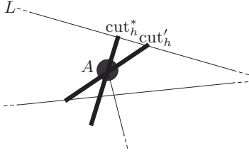
Fig. 14. Slide an endpoint of \text{cut}_h^* along L until it can no longer intersect the bottom link. This new cut is \text{cut}'_h .
