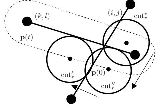
Fig. 18. A case in the proof of Lemma 9. \text{cut}_r^* is first translated in the direction of (i, j) to become \text{cut}_r'' which intersects (k, l) at exactly one point. Then \text{cut}_r'' is translated along \mathbf{p}(t) to \text{cut}_r' where (i, j) and (k, l) each intersect \text{cut}_r' at exactly one point.
