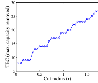
Fig. 25. The maximum value of TEC as a function of the cut radius for a circular cut in the fiber plant illustrated in Fig. 1.
