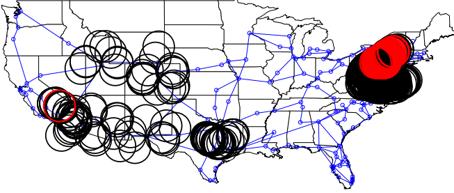
Fig. 23. The impact of circular cuts of radius 2 on the MFST between Los Angeles and NYC. Red circles represent cuts that result in MFST = 0 and black circles result in MFST = 1 . Cuts which intersect the nodes representing Los Angeles or NYC are not shown.
