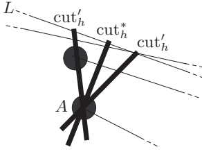
Fig. 13. Slide an endpoint of \text{cut}_h^* right along L until it intersects a link intersection. This new cut is the \text{cut}'_h on the right. We can also slide and endpoint of \text{cut}_h^* left along L until it intersects a node. This new cut is the \text{cut}'_h on the left.
