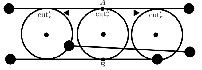
Fig. 16. A case in the proof of Lemma 9. Parallel links are tangent to \text{cut}_r'' at diametrically opposing points, A and B . Consider a translation of this cut such that it remains tangent to the two parallel links, intersects at least the same links as \text{cut}_r'' , and i) two links intersect only the boundary of this cut at distinct and non-diametrically opposing points or ii) two links intersect only the boundary of this cut and one of these intersection points is a node. Denote this translated cut by \text{cut}_r' . Now either \text{cut}_r' intersects the parallel links at exactly one point each where one of these points is a node, or \text{cut}_r' intersects two links at exactly one point each such that they are not diametrically opposite and distinct.
