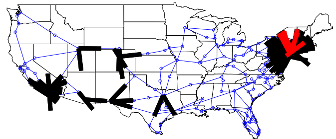
Fig. 21. Line segments cuts optimizing MFST between Los Angeles and NYC for h = 4 - the red cuts minimize MFST and the black lines are nearly worst-case cuts. Cuts which intersect the nodes representing Los Angeles or NYC are not shown.
