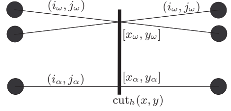
Fig. 7. Example showing (i_\omega, j_\omega) and (i_\alpha, j_\alpha) . (i_\alpha, j_\alpha) is the lowest link intersected by the cut and this intersection is at [x_\alpha, y_\alpha] . (i_\omega, j_\omega) are the highest links intersected by the cut and this intersection is at [x_\omega, y_\omega] . Note (i_\omega, j_\omega) is not unique.
