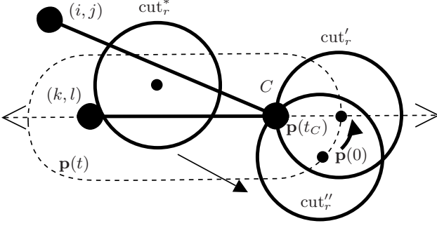
Fig. 17. A case in the proof of Lemma 9. \text{cut}_r^* is first translated in the direction of (i, j) to become \text{cut}_r'' which intersects only (k, l) at exactly one point and intersects another link (in this case (i, j) ) at exactly the same point. Then \text{cut}_r'' is translated along \mathbf{p}(t) towards \mathbf{p}(t_C) to \text{cut}_r' such that [x', y'] lies on the line which contains (k, l) .
