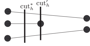
Fig. 10. \text{cut}_h' contains a node as well as intersects all links which \text{cut}_h^* does.
